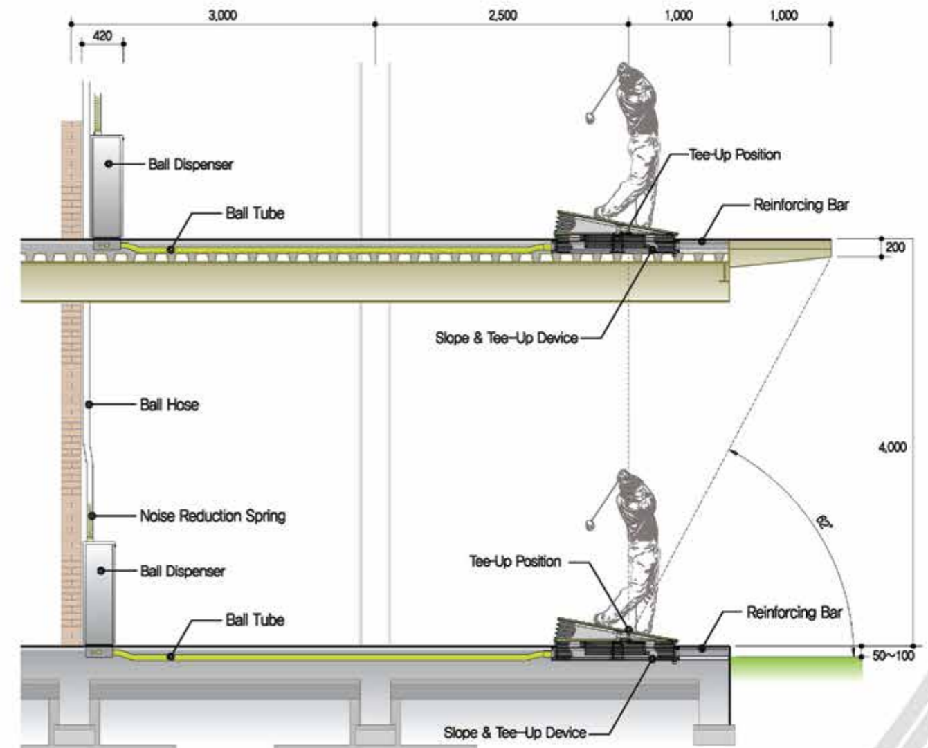
Cross-Sectional View
